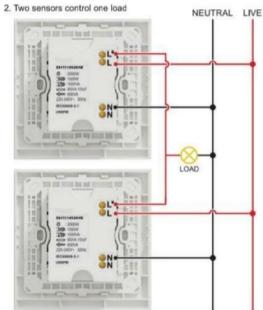
> PIR Motion Sensor* UNSPIR_WE
