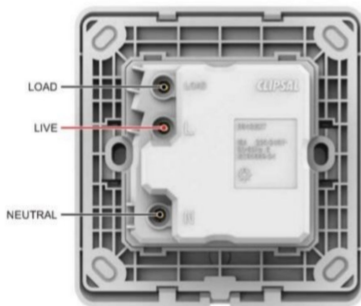
> 16A Electronic Keycard Switch CPXKEYCARDSW_WE, CPXKEYCARDSW_GY
