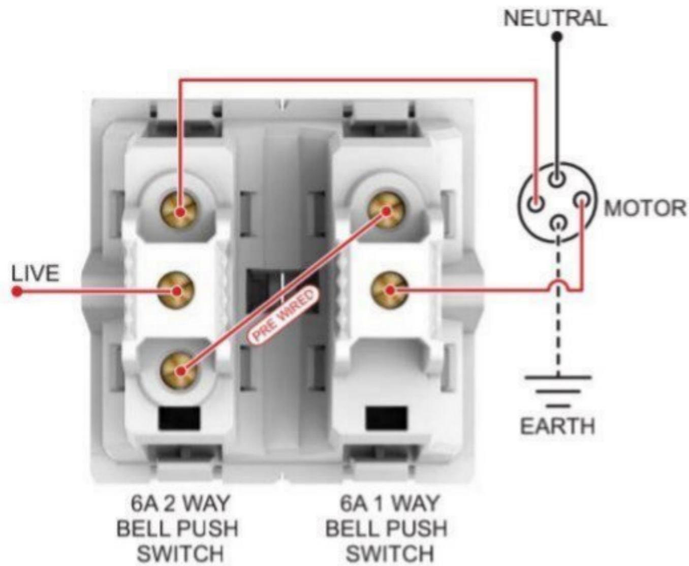
> Curtain Control Switch UNSCURTAINSW2M_WE
