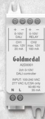
A2D0001 is a BLE-enabled 2 channel 0-10V or DALI controller. It has a universal 100-277V AC input voltage range and can control 2 separate analog channels, 1 Tunable White channel, or one Dali channel.
