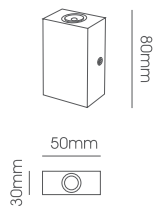
LLWL002-2*1W(TWO WAY) Body Size: 50*30*80mm
