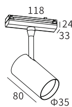
LMT001-6W Body Size :Ø35*80
