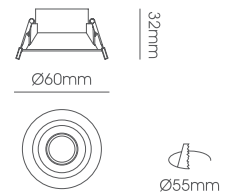
LLF263A Body Size: Ø60*32mm Cut-Size: Ø55mm
