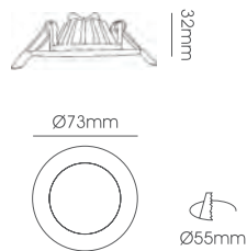
LLF035A-3W Body Size: Ø73*32mm Cut-Size: Ø55mm
