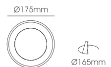
LLF058B-24W Body Size: Ø175*65mm Cut-Size: Ø165mm
