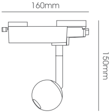
LLF277-6W Body Size: 160*150mm
