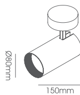
LLS073-20W Body Size: Ø80*150*157mm
