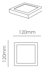
LLS005-6W Body Size: 120*120*35mm
