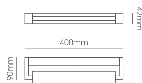
LLWL088-12W Body Size: 400*90*42mm
