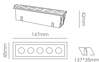
LLF259-12W Body Size: 147*45*42mm Cut-Size: 137*35mm
