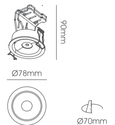
LLL066-9W Body Size: Ø78*90mm Cut-Size: Ø70mm
