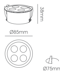
LLF257-10W Body Size: Ø85*38mm Cut-Size: Ø75mm
