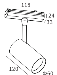
LMT003-18W Body Size :Ø60*120
