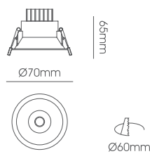
LLF278-7W Body Size: Ø70*65mm Cut-Size: Ø60mm
