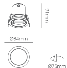
LLL098A-10W Body Size: Ø84*91mm Cut-Size: Ø75mm
