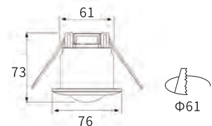
LMS 002-1200W/800W/300W/200W Body Size : \varnothing 76*73
