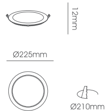
LLF010-22W Body Size: Ø225*12mm Cut-Size: Ø210mm
