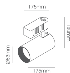
LLF159-40W Body Size: Ø83*175*180mm
