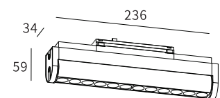
LMT105-12W Body Size :236*34*59
