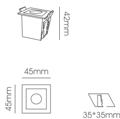
LLF256-3W Body Size: 45*45*42mm Cut-Size: 35*35mm
