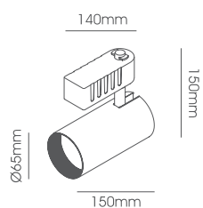
LLF157-20W Body Size: Ø65*150*150mm
