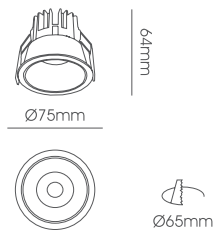
LLF110-9W Body Size: Ø75*64mm Cut-Size: Ø65mm
