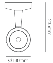
LLS038-30W Body Size: Ø130*235mm
