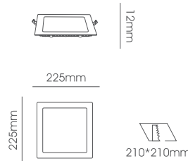
LLF015-22W Body Size: 225*225*12mm Cut-Size: 210*210mm
