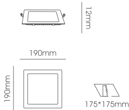
LLF014A-18W Body Size: 190*190*12mm Cut-Size: 175*175mm
