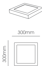
LLS008-24W Body Size: 300*300*35mm
