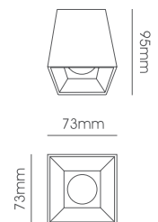
LLS047-12W Body Size: 73*73*95mm
