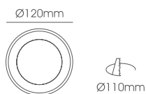
LLF058-12W Body Size: Ø120*55mm Cut-Size: Ø110mm
