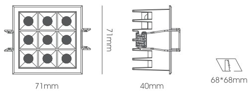
LLF214-12W Body Size: 71*71*40mm Cut-Size: 68*68mm
