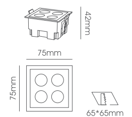
LLF258-10W Body Size: 75*75*42mm Cut-Size: 65*65mm
