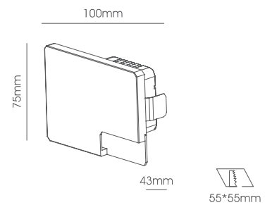
LLL122-3W Body Size: 100*75*43mm Cut-Size: 55*55mm
