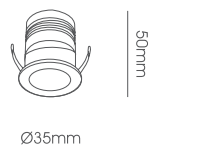
LLL067-3W Body Size: Ø35*50mm Cut-Size: Ø26mm
