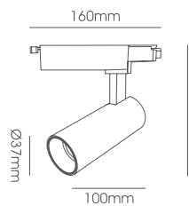
LLF159A-6W Body Size: Ø37*100*125*160mm
