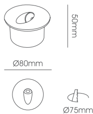
LLF163-1*3W Body Size: 80*50mm Cut-Size: 75mm
