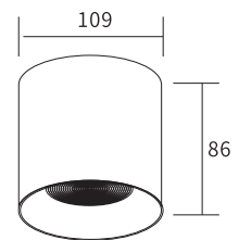
LLS 123A(SMD)-24W Body Size :Ø109*86
