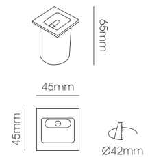
LLF162-1W Body Size: 45*65mm Cut-Size: 42mm
