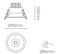
LLF280-20W Body Size: Ø95*100mm Cut-Size: Ø86mm
