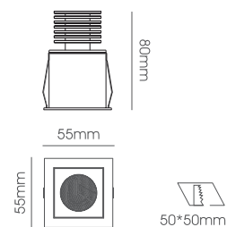
LLL034-5W Body Size: 55*55*80mm Cut-Size: 50*50mm
