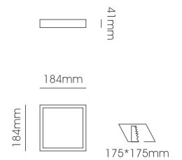
LLF006-22W Body Size: 184*184*41mm Cut-Size: 175*175mm
