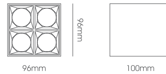
LLL094-15W Body Size: 96*96*100mm
