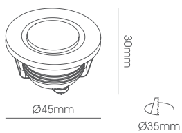
LLL120-1W Body Size: Ø45*109mm Cut-Size: Ø35mm
