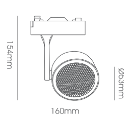
LLF231-10W Body Size: 160*Ø53*154mm
