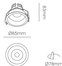
LLF237-15W Body Size: Ø85*83mm Cut-Size: Ø78mm
