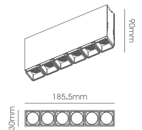
LLL020-6*2W Body Size: 185.5*30*90mm
