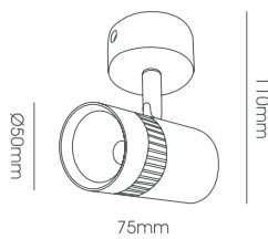
LLWL048A-3W Body Size: Ø50*75*110mm
