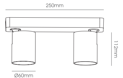
LLS087-SURFACE Body Size: Ø60*112mm Base Size: 250mm
