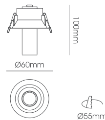
LLF264-5W Body Size: Ø60*100mm Cut-Size: Ø55mm
