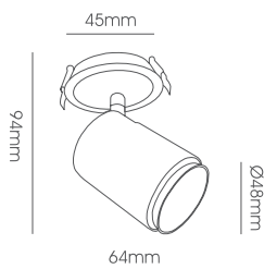
LLF226-3W Body Size: Ø48*64*94mm Cut-Size: Ø45mm
