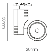
LLF149-10W Body Size: Ø80*120*150mm
