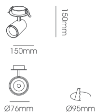
LLF202-16W Body Size: Ø76*150*150mm Cut-Size: Ø95mm
