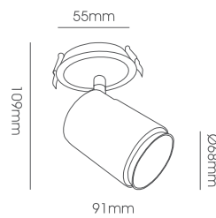
LLF227-6W Body Size: Ø68*91*109mm Cut-Size: Ø55mm
