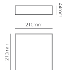
LLS062-20W Body Size: 210*210*44mm
