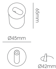
LLF160-1W Body Size: 45*65mm Cut-Size: 42mm
