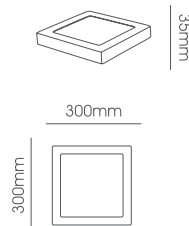
LLS008A-30W Body Size: 300*300*35mm
