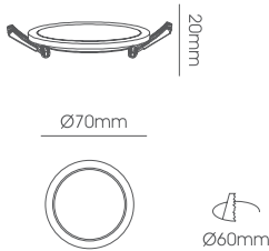
LLF040-4W Body Size: Ø70*20mm Cut-Size: Ø60mm
