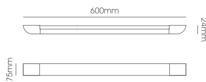
LLT010-20W Body Size: 600*75*24mm
