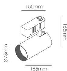
LLF158-30W Body Size: Ø73*165*165mm
