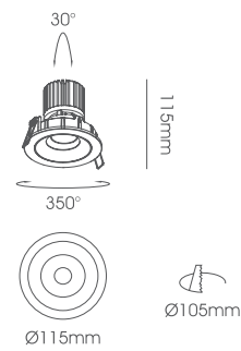
LLL097-12W Body Size: Ø115*115mm Cut-Size: Ø105mm
