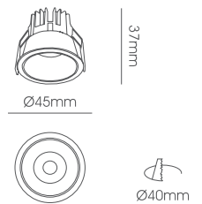
LLF112-3W Body Size: Ø45*37mm Cut-Size: Ø40mm
