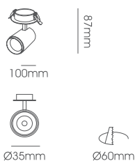
LLF200-5W Body Size: Ø35*100*87mm Cut-Size: Ø60mm
