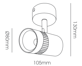
LLWL048C-9W Body Size: Ø80*105*130mm
