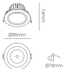
LLF073-9W Body Size: Ø85*74mm Cut-Size: Ø78mm
