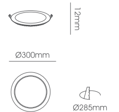
LLF011-30W Body Size: Ø300*12mm Cut-Size: Ø285mm
