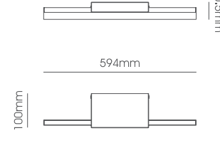
LLT021-12W Body Size: 594*100*50,5mm
