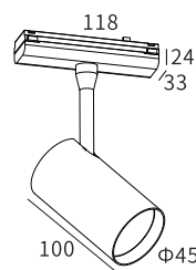
LMT002-12W Body Size :Ø45*100
