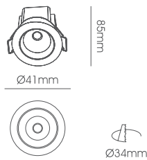
LLF275-7W Body Size: Ø41*85mm Cut-Size: Ø34mm
