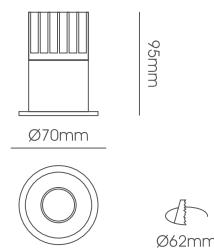
LLF273-12W Body Size: Ø70*95mm Cut-Size: Ø62mm
