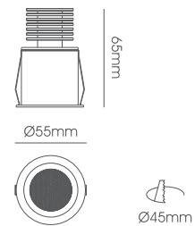
LLL084A-10W Body Size: Ø55*65mm Cut-Size: Ø45mm
