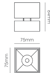
LLS085-8W Body Size: 75*75*84mm
