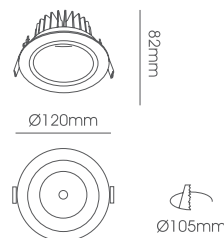
LLF074-16W Body Size: Ø120*82mm Cut-Size: Ø105mm
