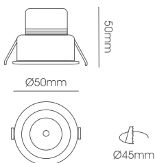
LLF063-5W Body Size: Ø50x50mm Cut-Size: Ø45mm
