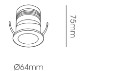
LLL069-12W Body Size: Ø64*75mm Cut-Size: Ø55mm
