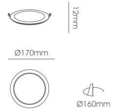
LLF009-12W Body Size: Ø170*12mm Cut-Size: Ø160mm
