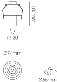
LLF242-8W Body Size: Ø74*100mm Cut-Size: Ø65mm
