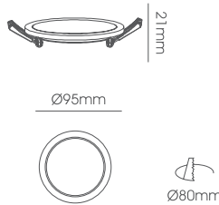
LLF050-8W Body Size: Ø95*21mm Cut-Size: Ø80mm
