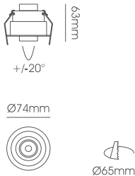
LLF241-5W Body Size: Ø74*63mm Cut-Size: Ø65mm
