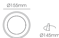
LLF058A-18W Body Size: Ø155*65mm Cut-Size: Ø145mm
