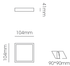
LLF004-8W Body Size: 104*104*41mm Cut-Size: 90*90mm
