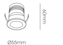
LLL068-6W Body Size: Ø55*60mm Cut-Size: Ø46mm
