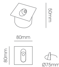
LLF164-1*3W Body Size: 80*50mm Cut-Size: 75mm
