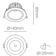
LLF075-30W Body Size: Ø140*80mm Cut-Size: Ø125mm
