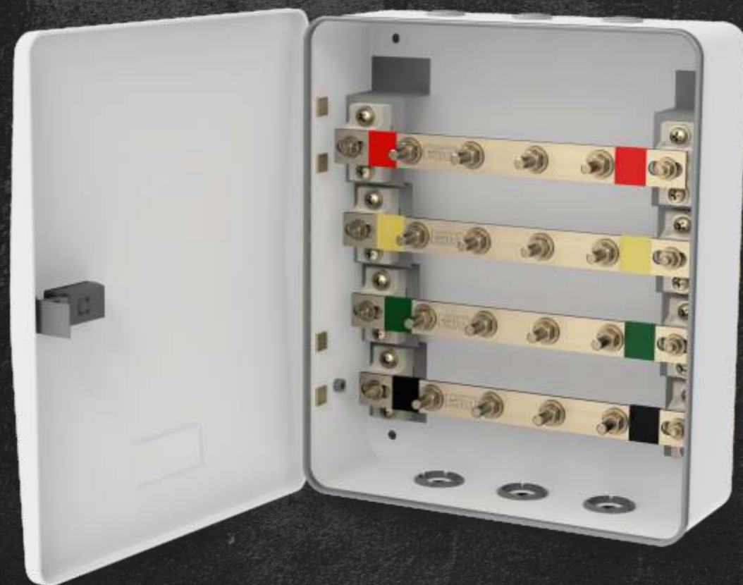
Busbar Chamber
